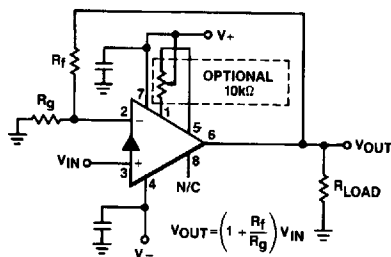
EL2020 Typical Non-Inverting Amplifier Characteristics
